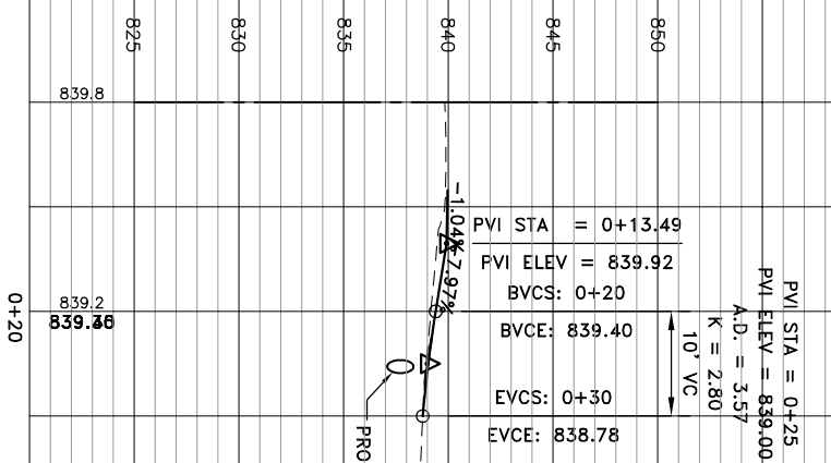
DRIVE PROFILE STATION 13+52.55 LT
